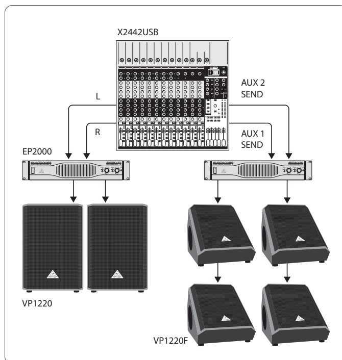
Fig. 5.2: Full-range stereo operation with floor monitors
